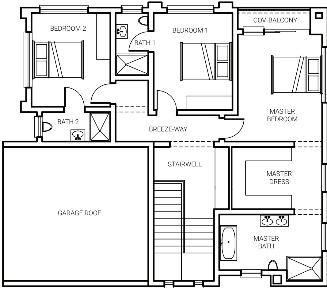
FIRST FLOOR UNIT 1, 3, 5 & 7
