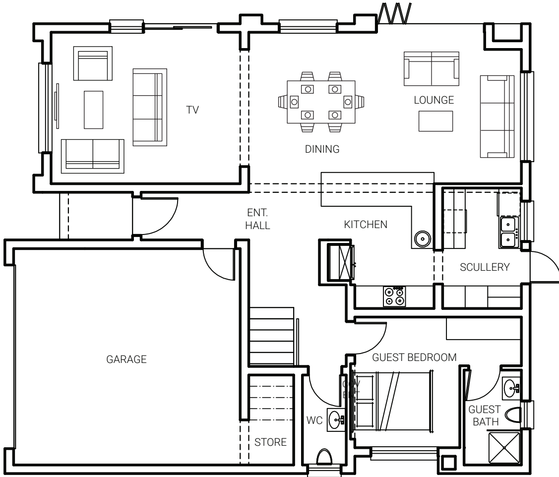
GROUND FLOOR UNIT 1, 3, 5 & 7
