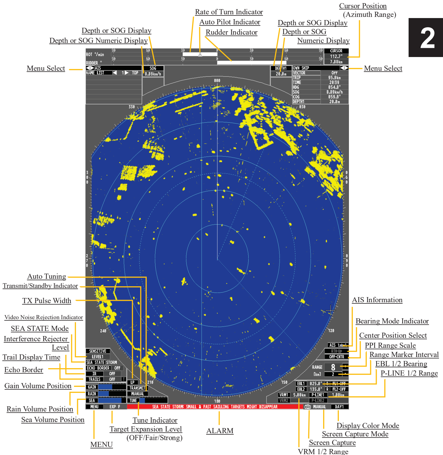
FIG 2.1 DISPLAY & READOUTS
