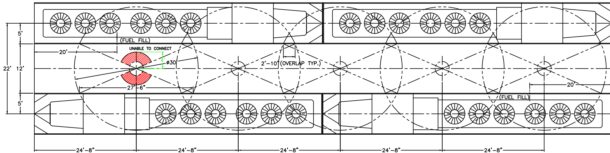
104-HP-1 FUEL CRANE SPACING EXAMPLE
