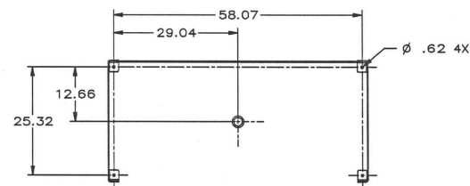
SECTION A-A ANCHOR BOLT PATTERN
