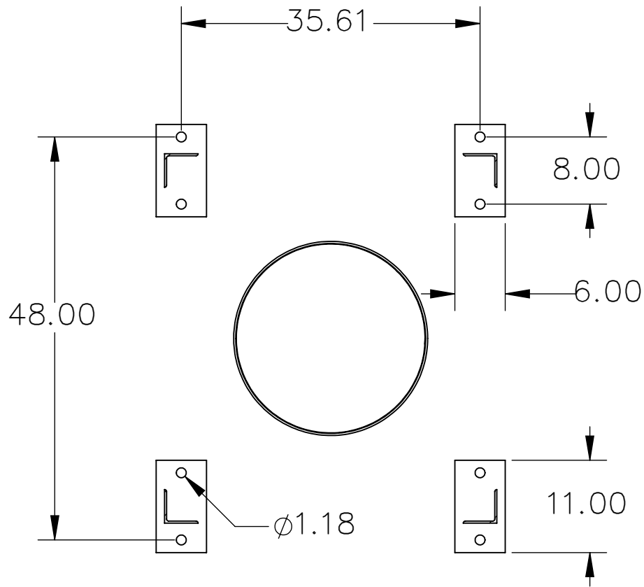
SECTION A-A ANCHOR BOLT PLAN
