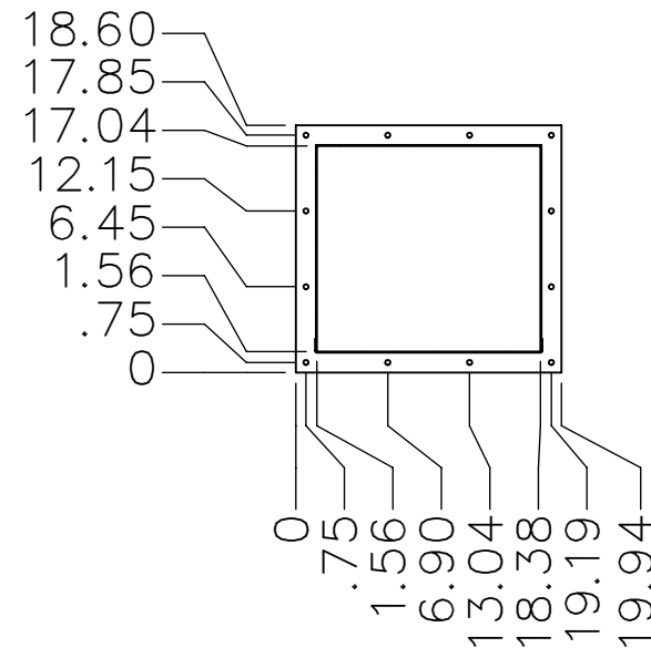
SECTION B-B SILENCER OUTLET FLANGE
